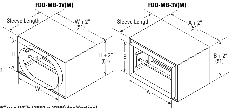
A= Duct Width B= Duct Height
