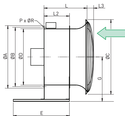
Support frame, inlet cone and wire guard for AZN
