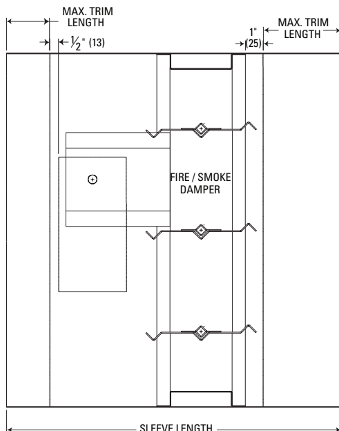
Figure 2 Combination Fire/Smoke Damper
